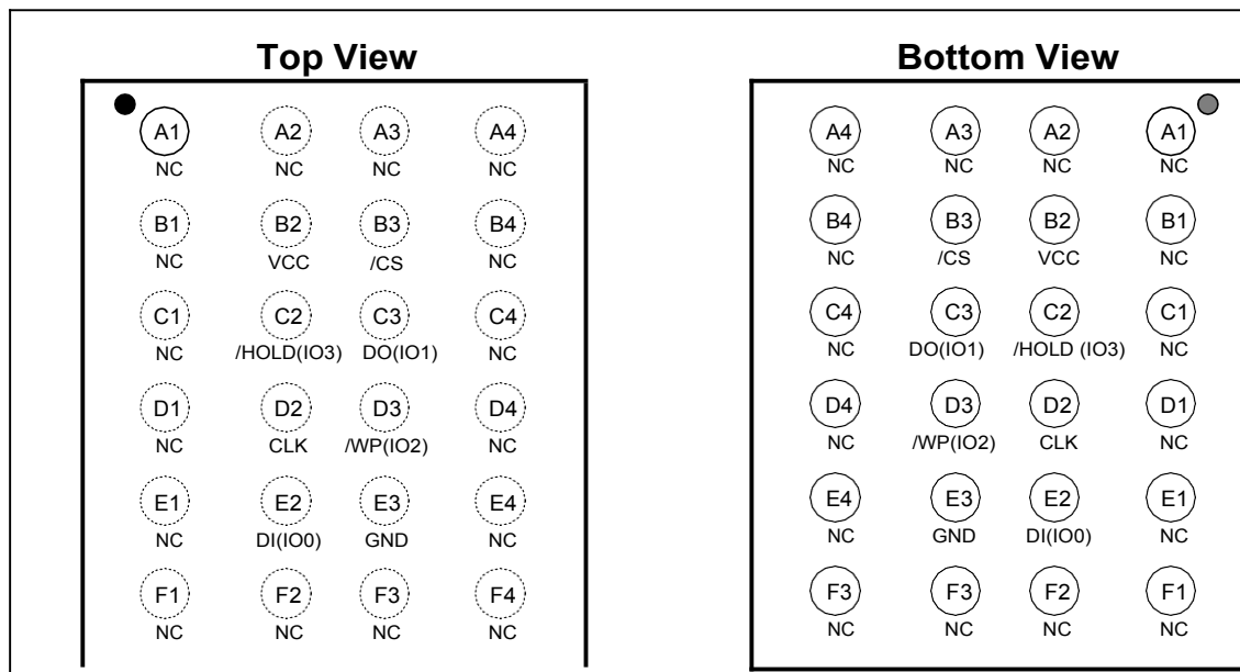
Figure 1e. W25Q128JV Ball Assignments, 24-ball WLCSP (Package Code Y)
