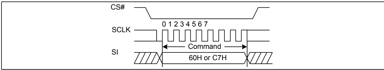
Figure20. Chip Erase Sequence Diagram
