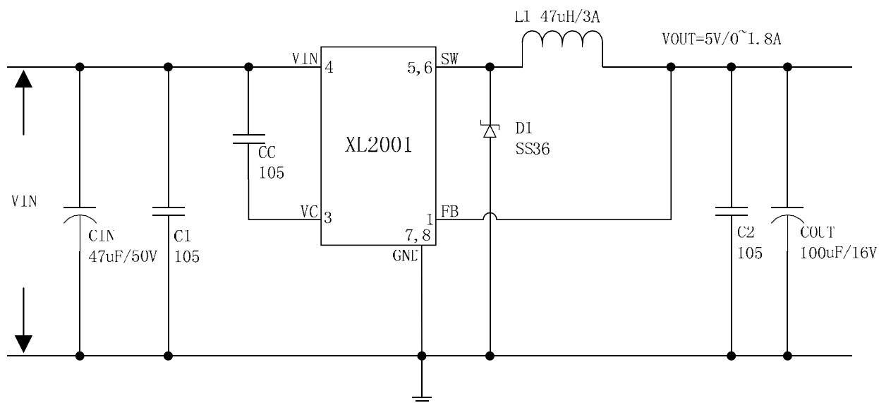
Figure4. XL2001 Typical Application Circuit ( V_{IN}=8V\sim 45V , V_{OUT}=5V/1.8A )
