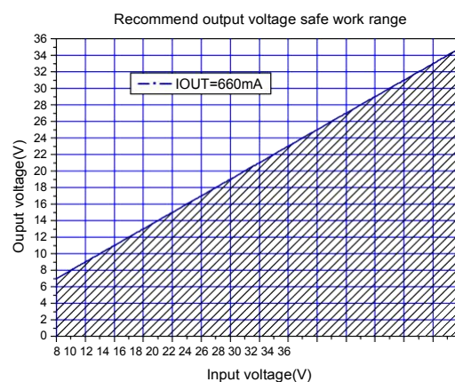
Figure13.Max output voltage(IOUT=660mA)
