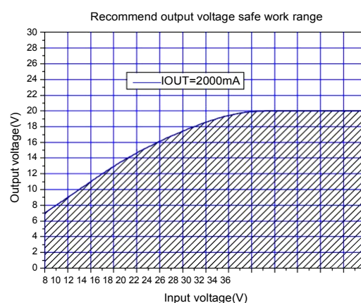
Figure15.Max output voltage(IOUT=2000mA)
