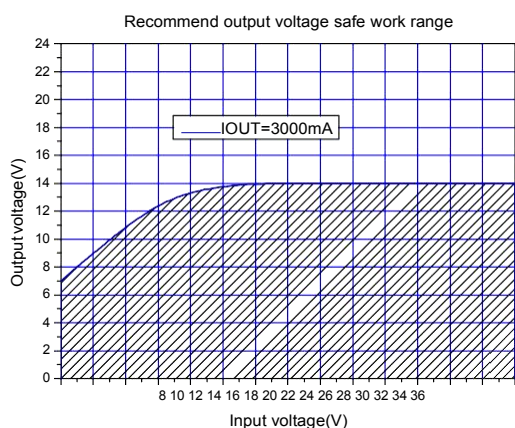
Figure16.Max output voltage(IOUT=3000mA)
