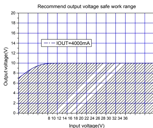
Figure17.Max output voltage(IOUT=4000mA)
