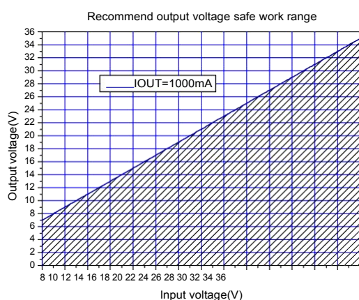
Figure14.Max output voltage(IOUT=1000mA)
