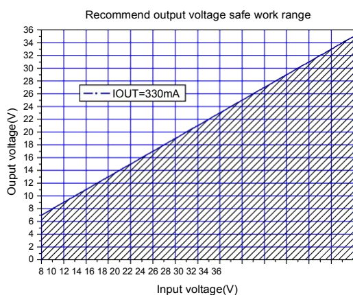
Figure12.Max output voltage(IOUT=330mA)
