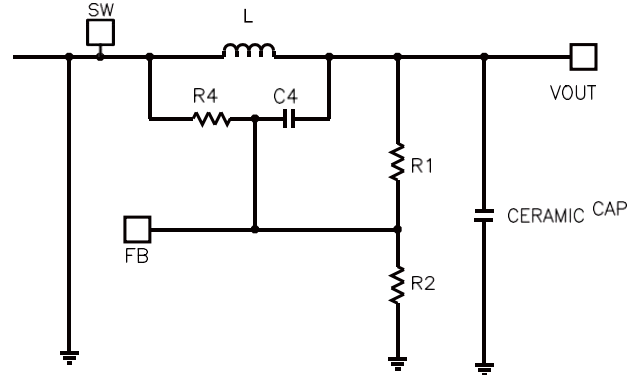
Figure 5—Simplified Circuit in PWM Mode with External Ramp Compensation
