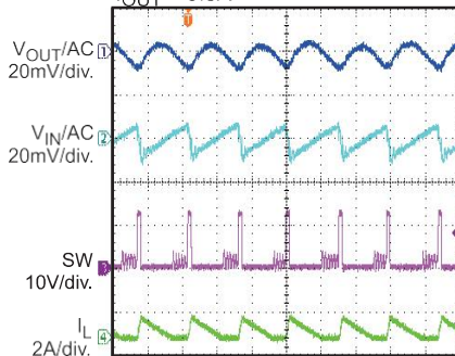
Input/Output Voltage Ripple
