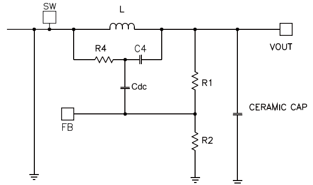
Figure 3—Simplified Circuit of External Ramp Compensation with DC blocking capacitor.
