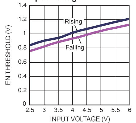
EN Threshold vs. Input Voltage
