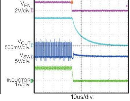
Power-Down Through EN
