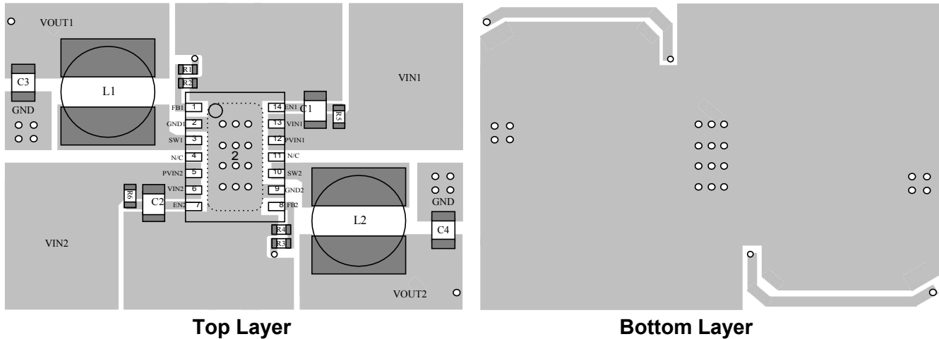
Figure 3 -PCB Layout
