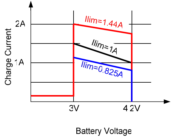
Figure 7— I_{CHG} Variation with Different Input Current Limit
