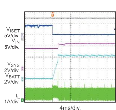
Charge On
