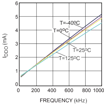
I_{DDO} Operation Current vs. Frequency
