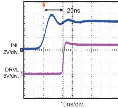
Turn-on Propagation Delay
