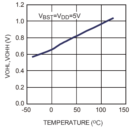
High Level Output Voltage vs. Temperature
