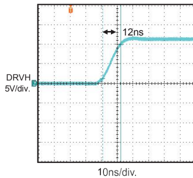
Drive Rise Time (1nF Load)
