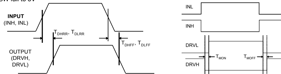
Figure 1—Timing Diagram
