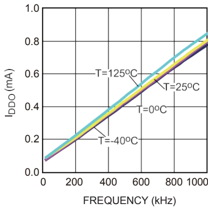
I_{DDO} Operation Current vs. Frequency
