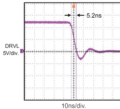
Drive Fall Time (1nF Load)
