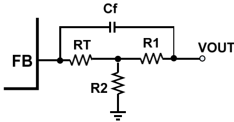
Figure 6: T-Type Network
