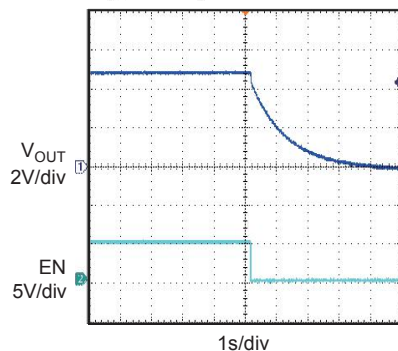
Turn Off Delay and Fall Time with 0.1 \mu F Load
