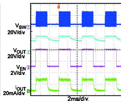
PWM DIM
