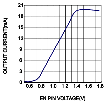
Analog DIM Curve
