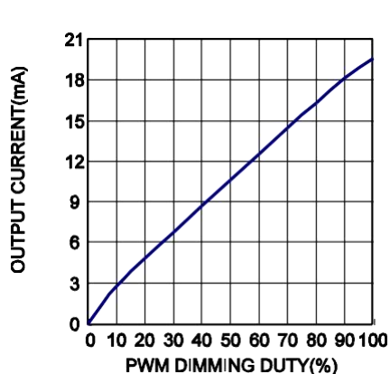
PWM Dim Curve
