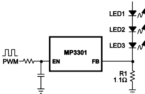
Figure 3: Control Circuit for High-Frequency PWM Dimming
