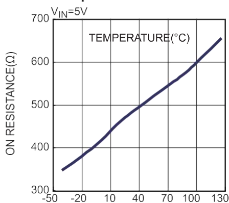
Bridge A HS ON RESISTANCE vs. Temperature
