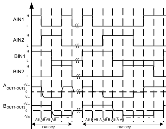
Figure 7: Signal Logic Sequences for Full-Step and Half-Step
