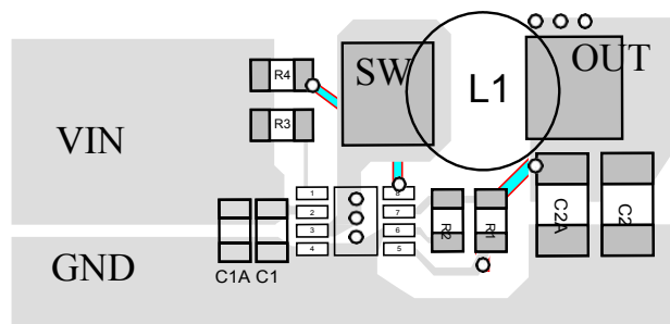
Figure 3: Layout Recommendation
