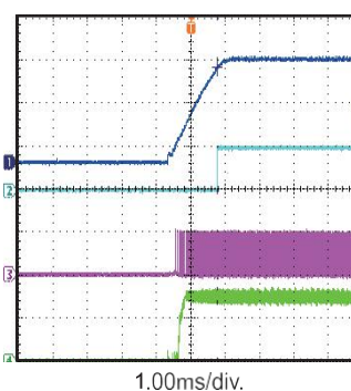
Power Good On with 2A Load
