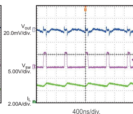
Output Ripple
