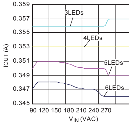
Line/Load Regulation
