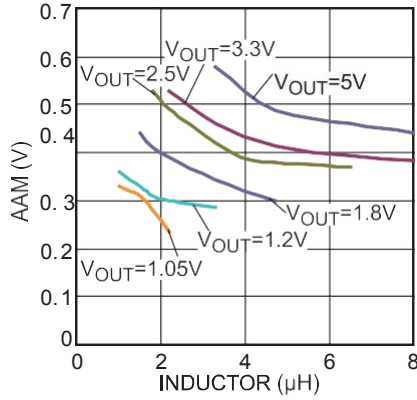
Figure 6— AAM Selection for Common Output Voltages (VIN=4.5V-24V) Selecting the Input Capacitor
