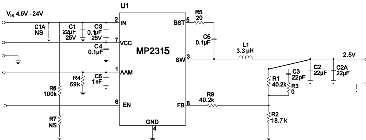
Figure 11: Vo=2.5V, Io=3A
