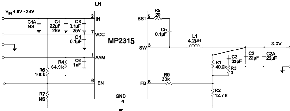
Figure 10: Vo=3.3V, Io=3A
