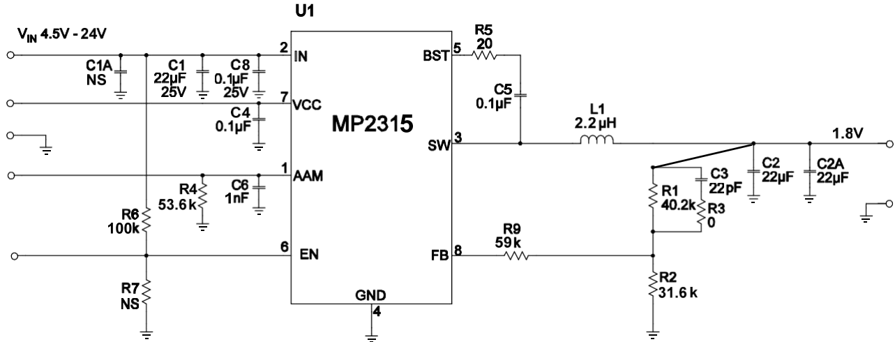
Figure 12: V_o=1.8V , I_o=3A
