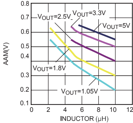
Figure 6: AAM Values for Common Output Voltages (VIN = 4.5V to 16V)
