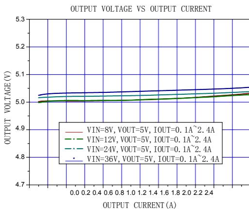
Figure9. Line & Load regulation Curve
