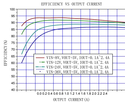
Figure8. Efficiency Curve
