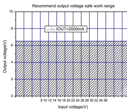
Figure15.Max output voltage(IOUT=2000mA)
