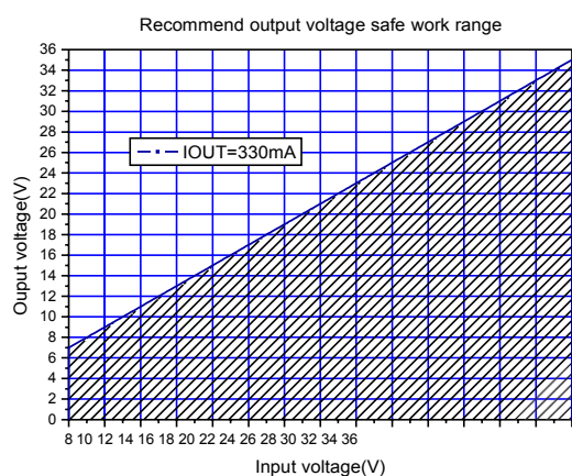
Figure12.Max output voltage(IOUT=330mA)
