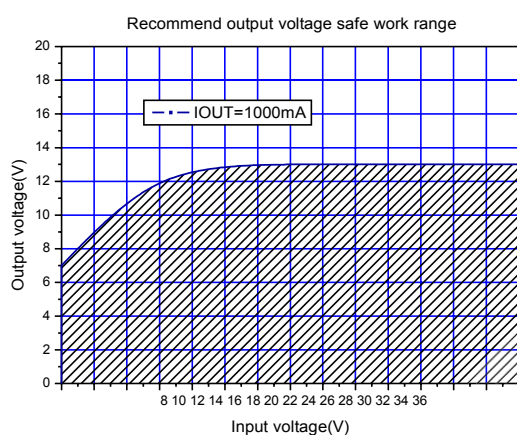
Figure14.Max output voltage(IOUT=1000mA)
