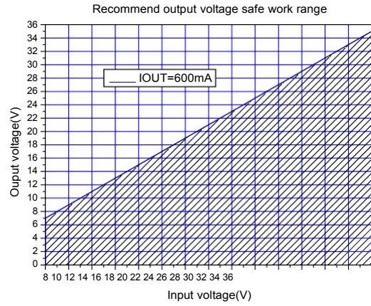
Figure6.Max output voltage(IOUT=600mA)
