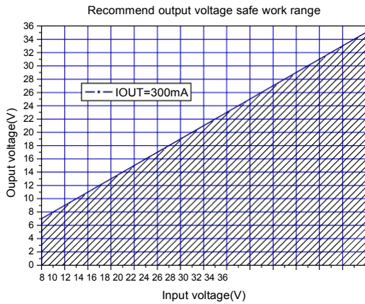
Figure5.Max output voltage(IOUT=300mA)
