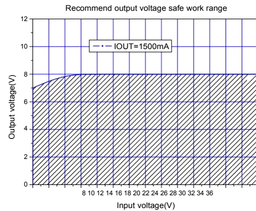
Figure8.Max output voltage(IOUT=1500mA)
