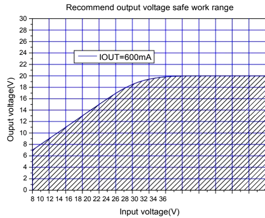
Figure6.Max output voltage(IOUT=600mA)
