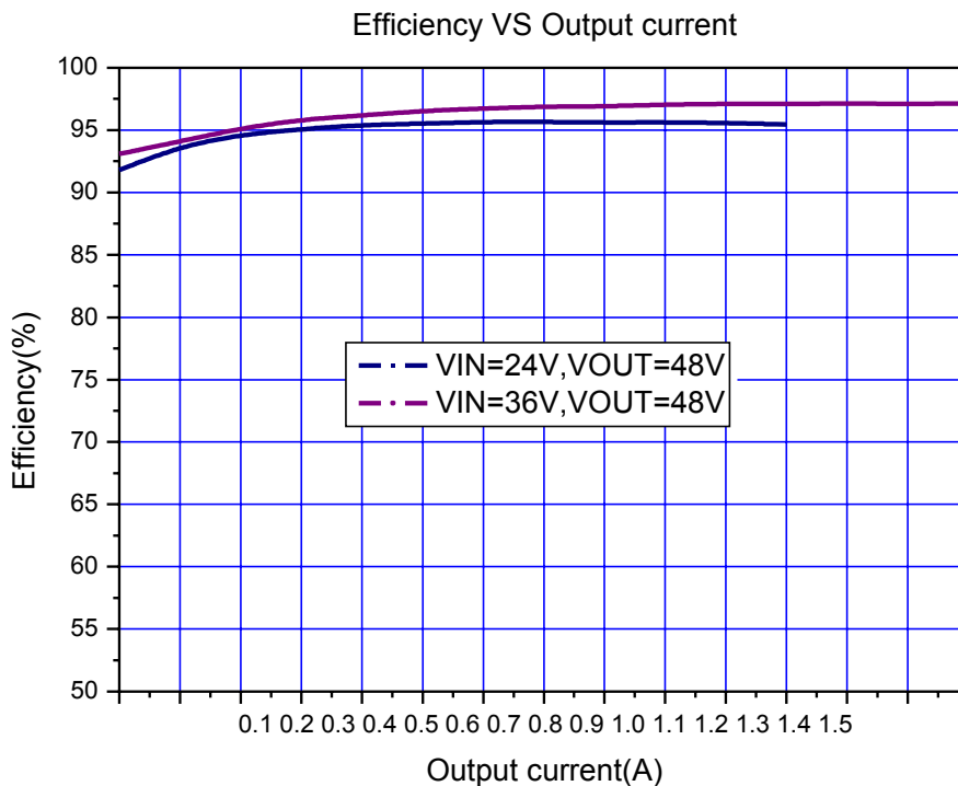
Figure18. XL6012 System Efficiency Curve (VIN=20~40V, VOUT=48V)
