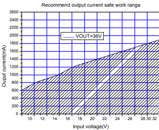
Figure7.Max output current (VOUT=36V)
