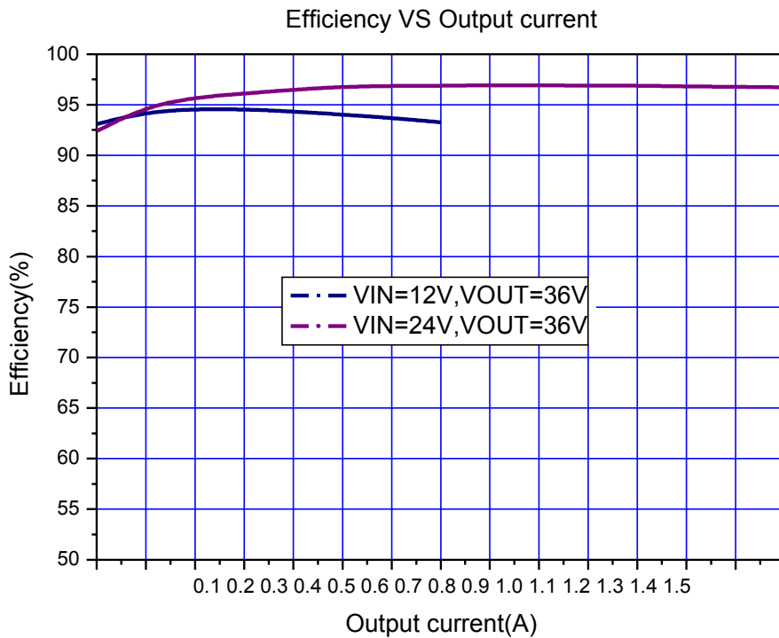
Figure16. XL6012 System Efficiency Curve (VIN=10~32V, VOUT=36V)
