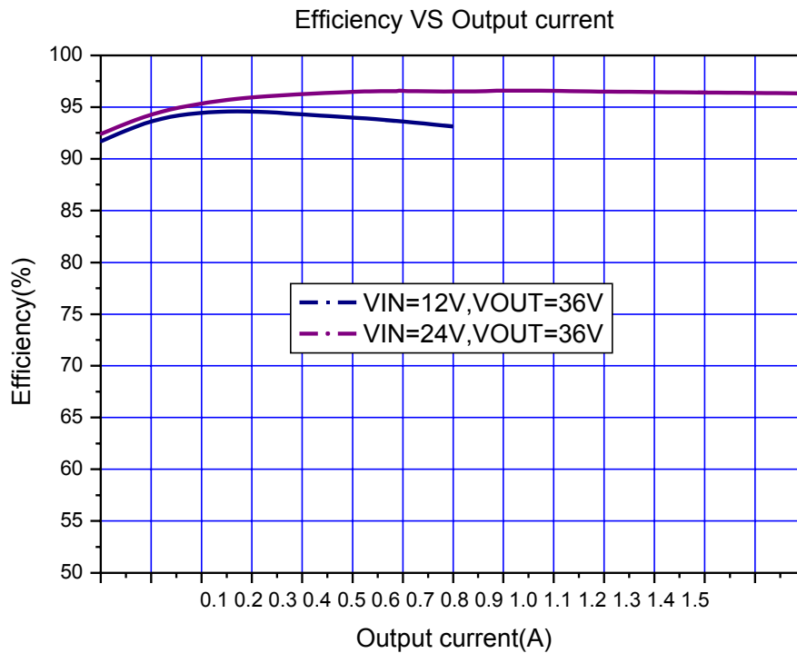
Figure14. XL6019 System Efficiency Curve (VIN=10~32V, VOUT=36V)
