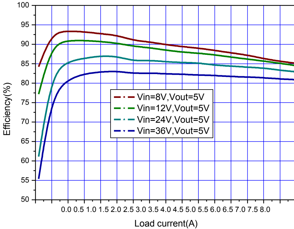
Figure6. XL4016 System Efficiency Curve
