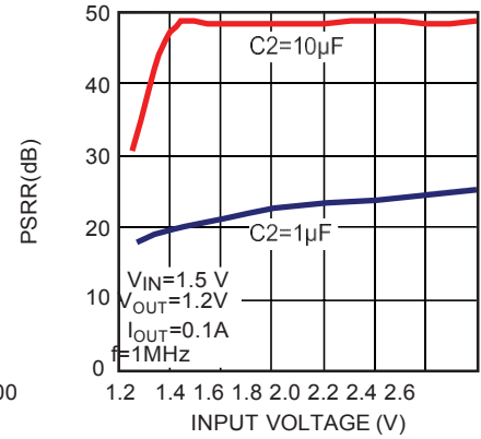
PSRR vs. V_{\text{IN}}
