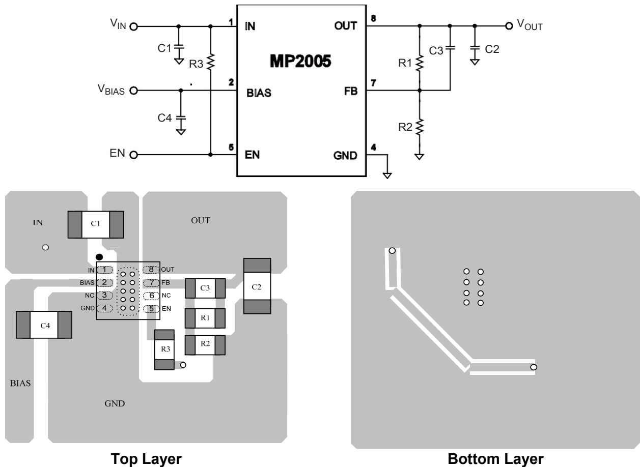
Figure 2—PCB Layout
