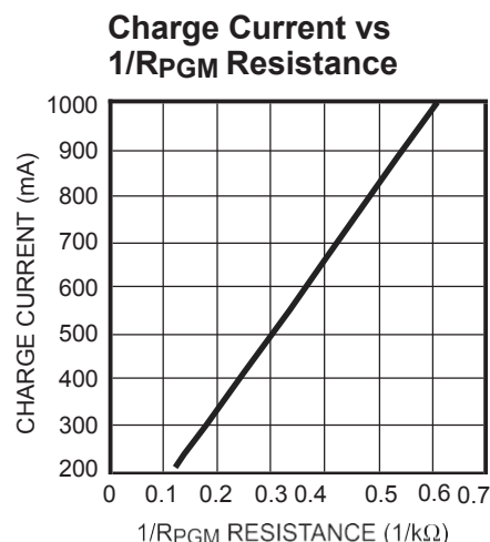
Figure 4—Charge Current vs 1/R_{PGM} Resistance
