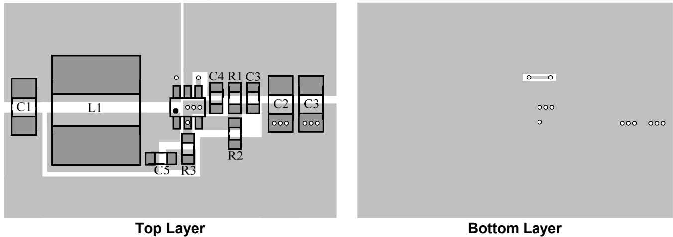
Figure3—PCB Layout
