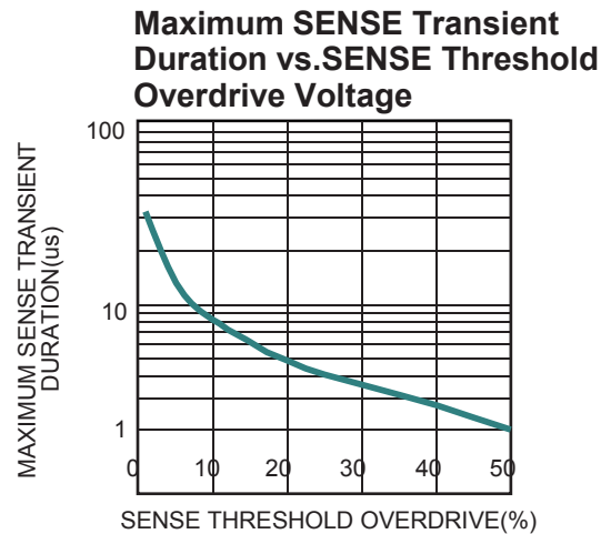
Figure 8—Maximum Transient Duration vs. Sense Threshold Overdrive Voltage
