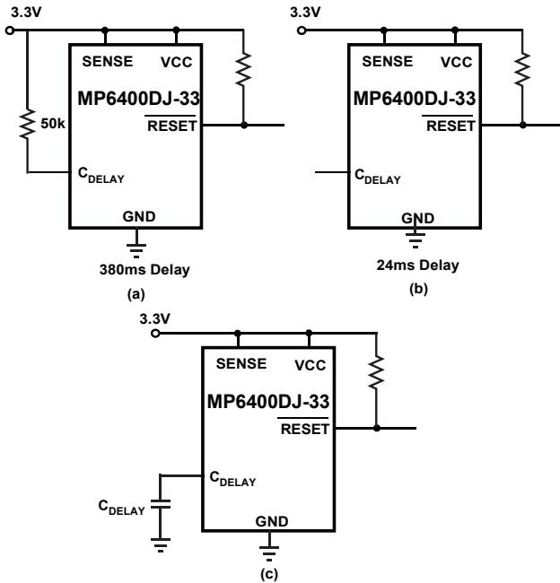
Figure 7—Programmable Configurations to the Reset Delay Time
