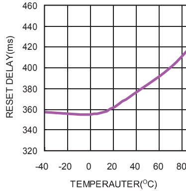
Reset Delay vs. Temperature ( C_{DELAY}=V_{CC} )
