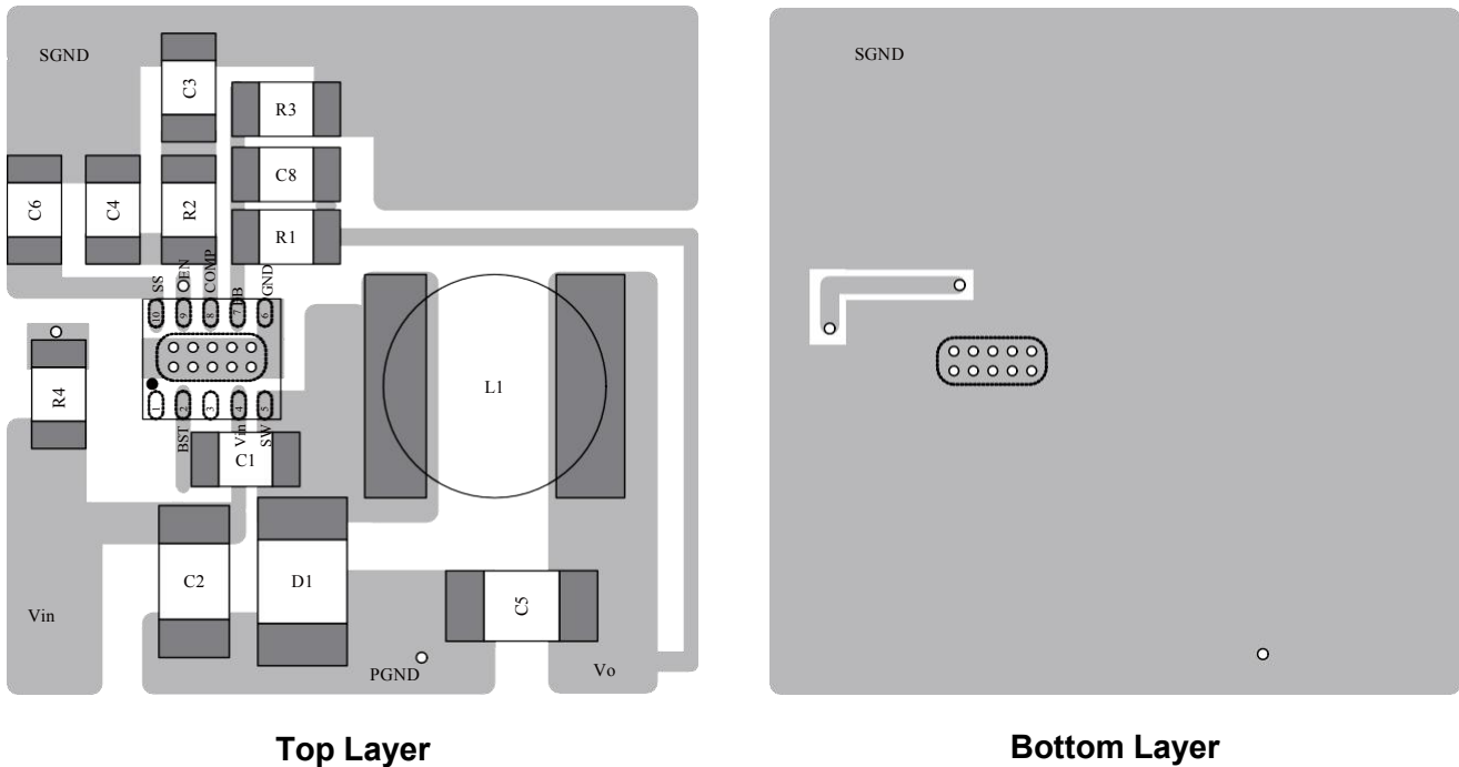
Figure3—PCB Layout
