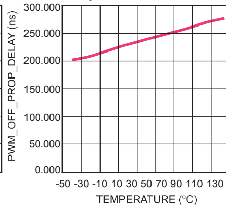
PWM Dimming Off Propagation Delay Time vs. Temperature
