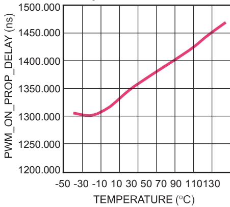
PWM Dimming On Propagation Delay Time vs. Temperature
