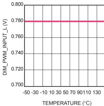
PWM Low High Threshold vs. Temperature
