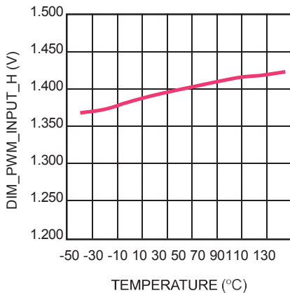
PWM Input High Threshold vs. Temperature
