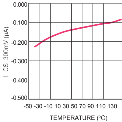
CS Pin Current vs. Temperature V CS =0.3V
