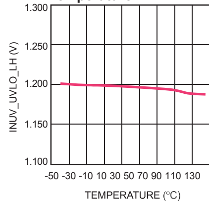
Input Bus Voltage UVLO Threshold vs. Temperature
