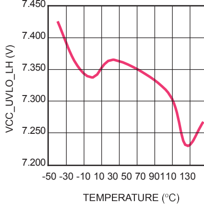
VCC UVLO vs. Temperature
