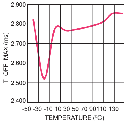
Maximum Off Time vs. Temperature
