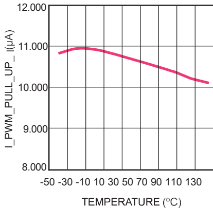
PWM Pull Up Current vs. Temperature
