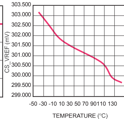
CS Reference Voltage vs. Temperature
