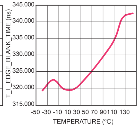
Leading Edge Blanking Time vs. Temperature
