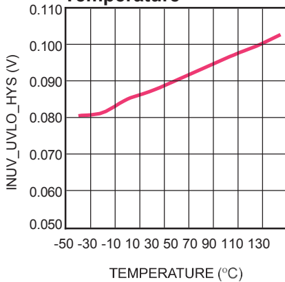
Input Bus Voltage UVLO Hysteresis vs. Temperature
