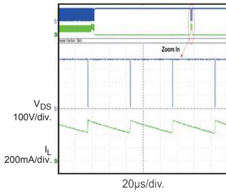
Open Loop
