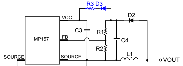
Figure 9: Auxiliary V CC Supply Circuit
