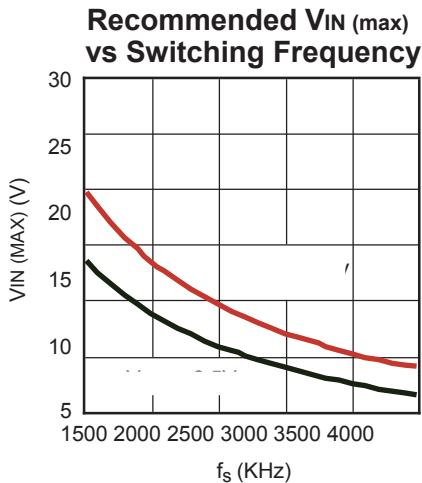
Figure 2—Recommend Max V_{IN} vs. f_s
