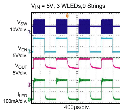
PWM Dimming
