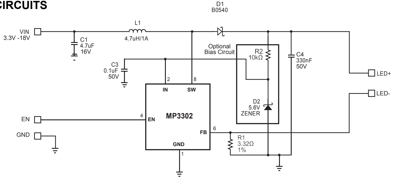
Figure 5 — Driving 27 WLEDs (9 WLEDs in Series and 3 Strings Paralleled) with 3.3V—18V Input Voltage
