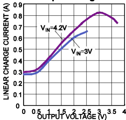
Linear Charge Current vs. Output Voltage
