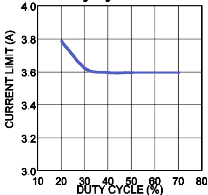
Boost Current Limit vs. Duty Cycle
