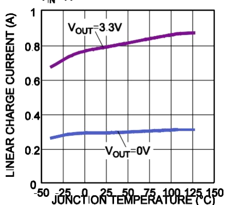
Linear Charge Current vs. Junction Temperature V_{IN} = 4V
