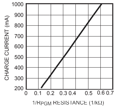
Figure 4—Charge Current vs 1/R_{PGM} Resistance
