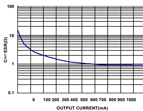
Figure 2—Relationship between ESR and LDO Stability
