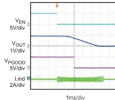
PGOOD, Shutdown Through EN
