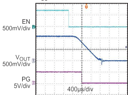
Power Good Through EN Shut Down
