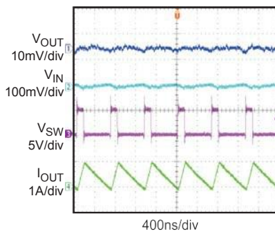
Steady State
