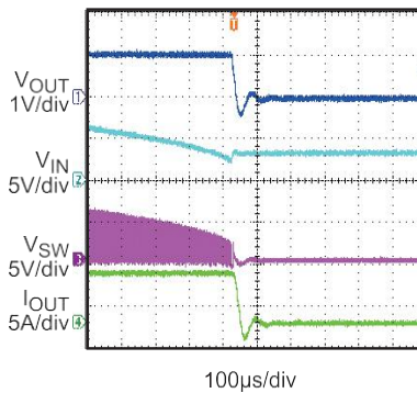
Shut Down Through VIN
