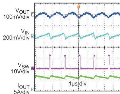
Input/Output Voltage Ripple
