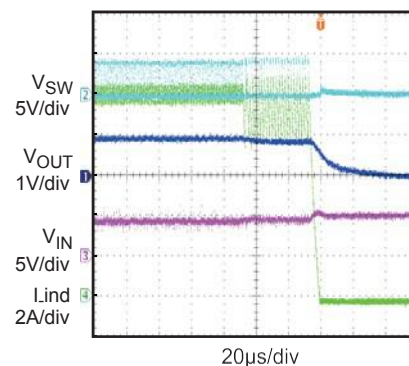
Over-current Protection
