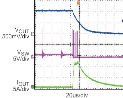
Short-Circuit Protection
