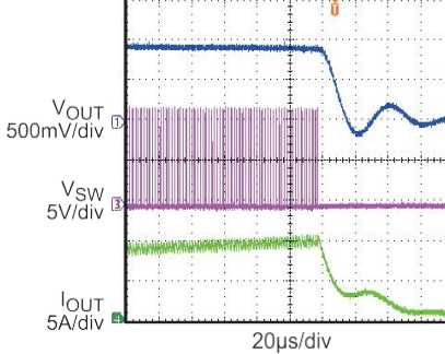
Over-Current Protection
