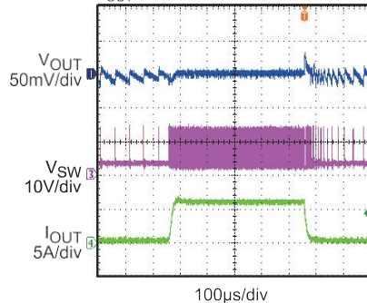
Transient Response
