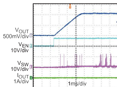
Start Up Through EN
