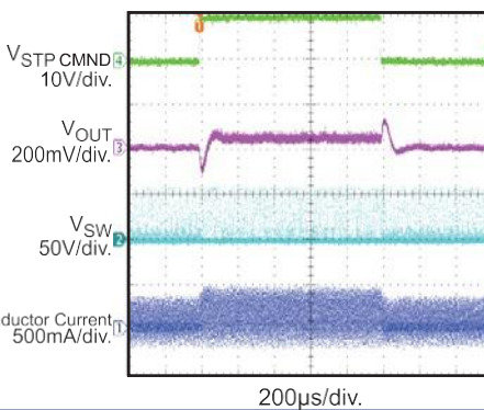
Transient Response 0.5mA to 2mA
