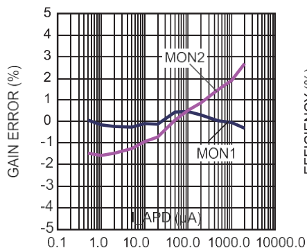
Gain Error vs. APD Current
