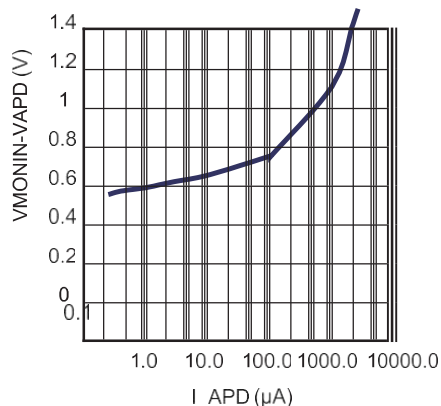
Voltage Drop - Vmonin to Vapd
