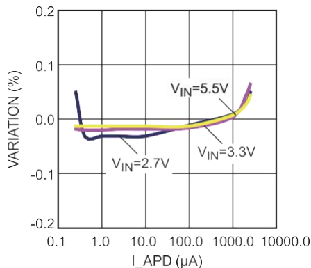
Load Regulation
