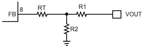
Figure 4: T-Type Network
