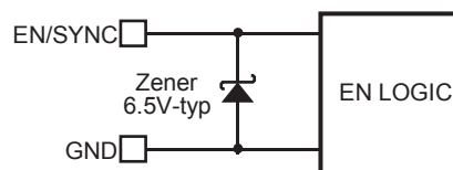
Figure 2: Zener Diode Circuit
