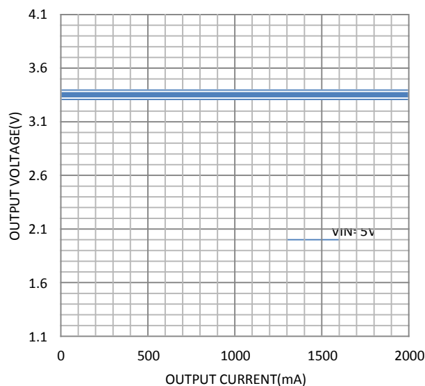
OUTPUT VOLTAGE VS OUTPUT CURRENT (VOUT=3.3V)
