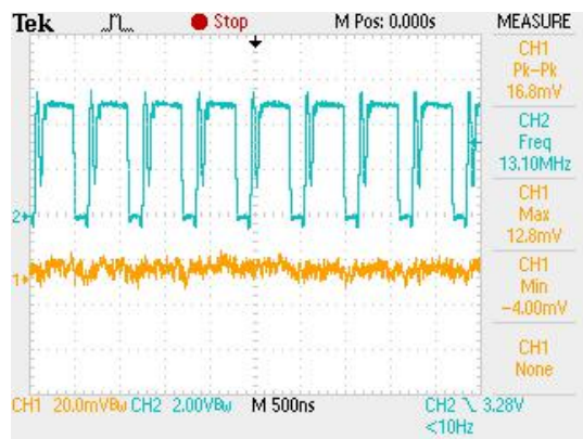
STEADY STATE OPERATION (VIN=5V, VOUT=3.3V, IOUT=100mA)
