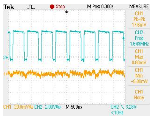
STEADY STATE OPERATION (VIN=5V, VOUT=3.3V, IOUT=1500mA)
