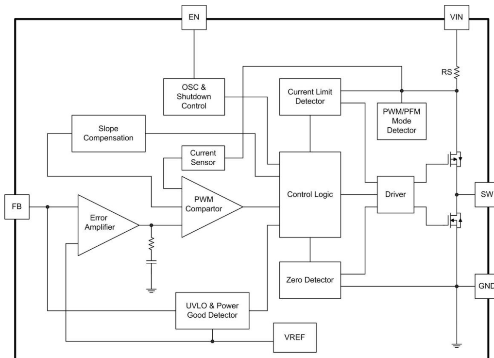
Figure 1. TX9406B Block Diagram
