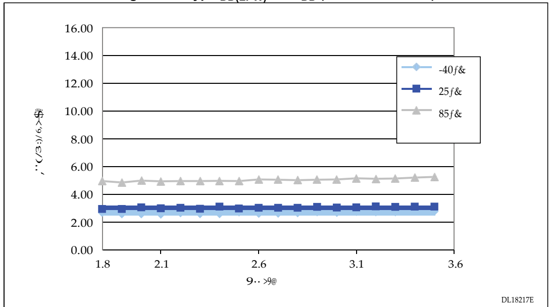
Figure 16. Typ. I_{DD(LPW)} vs. V_{DD} (LSI clock source)
