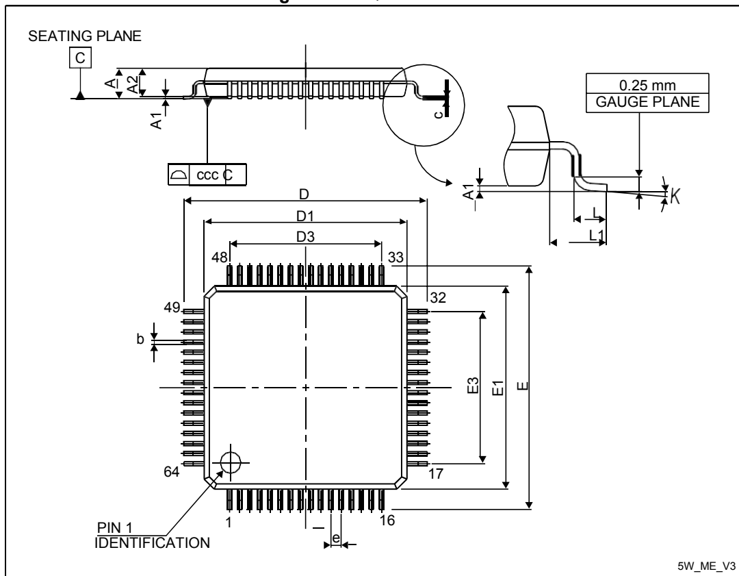
Figure 28. LQFP64 outline
