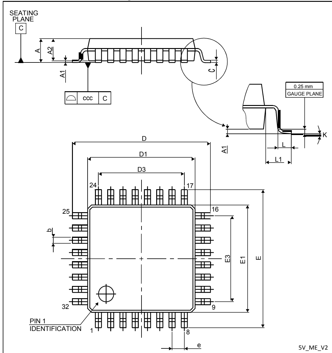
Figure 34. LQFP32 outline
