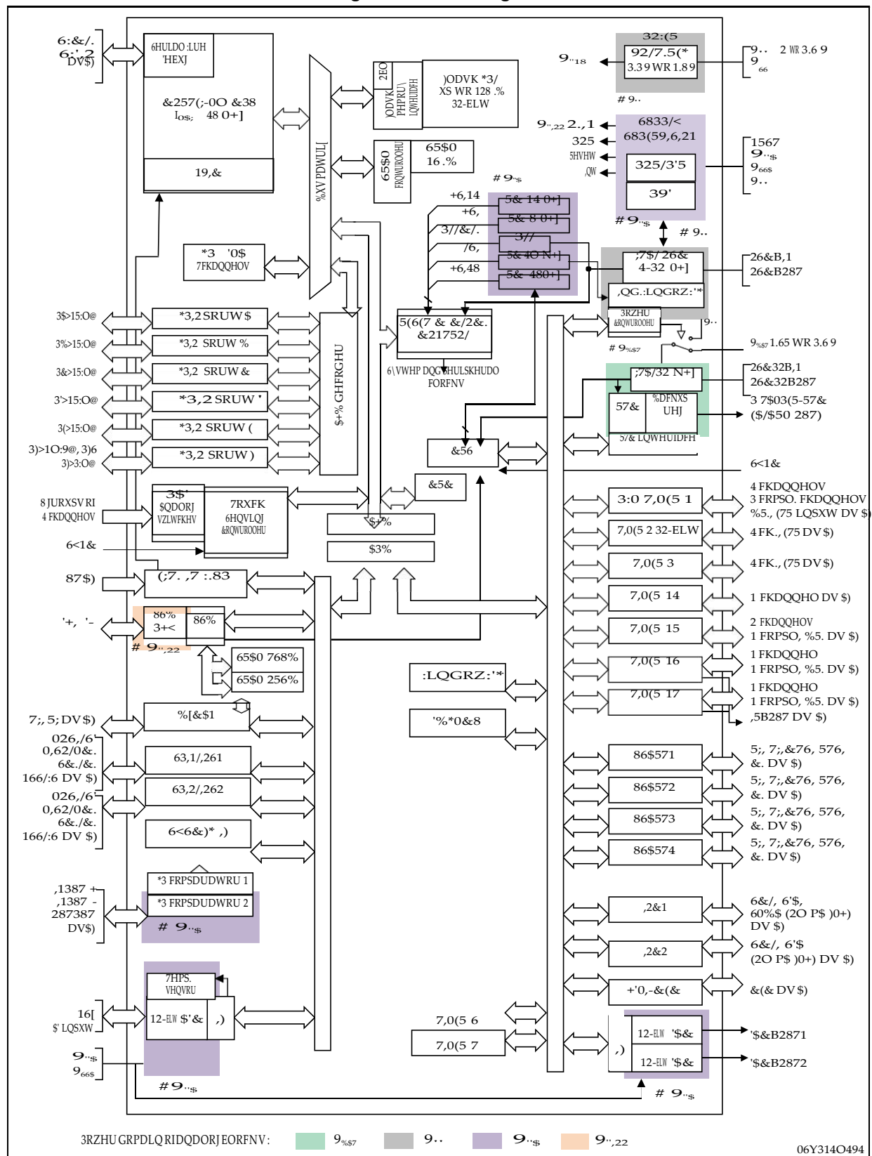
Figure 1. Block diagram
