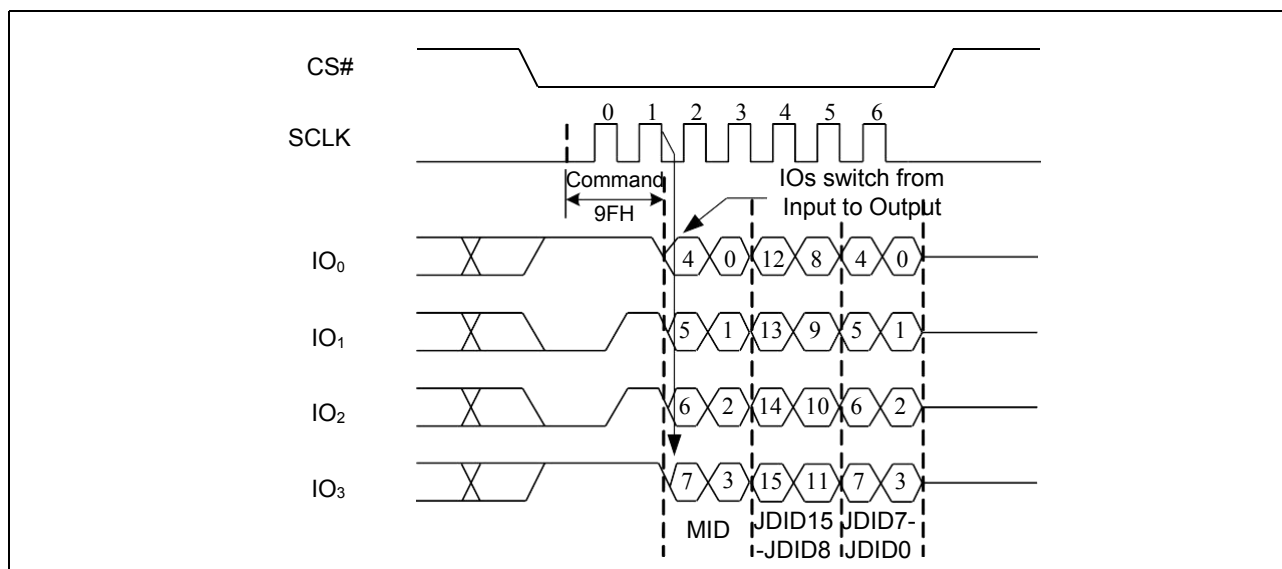
Figure28a. Read Identification ID Sequence Diagram (QPI)
