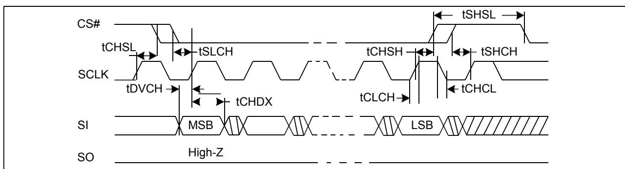
Figure49. Serial Input Timing
