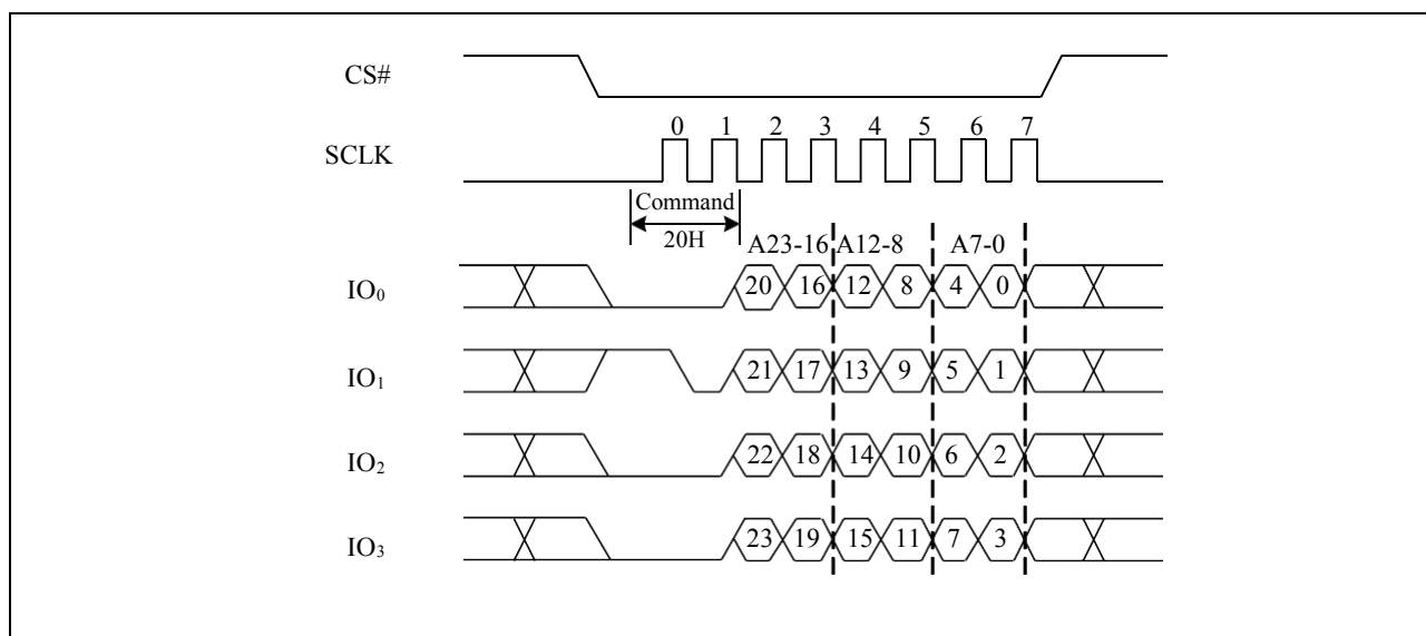
Figure18a. Sector Erase Sequence Diagram (QPI)
