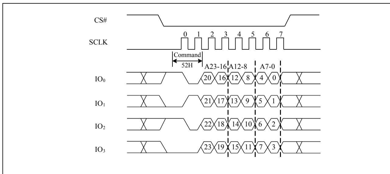
Figure19a. 32KB Block Erase Sequence Diagram (QPI)
