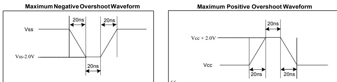
Figure 47. Maximum Negative/positive Overshoot Diagram
