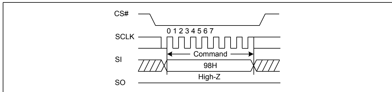
Figure38. The Global Block/Sector Unlock Sequence Diagram
