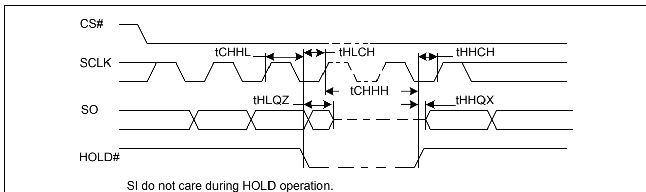
Figure51. Hold Timing
