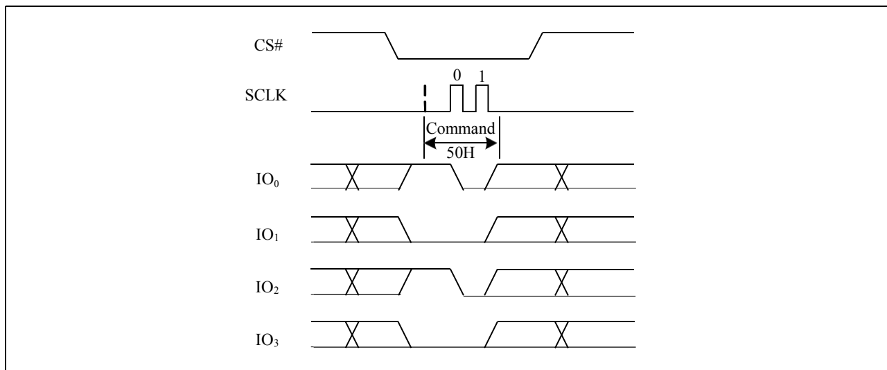
Figure5a. Write Enable for Volatile Status Register Sequence Diagram (QPI)
