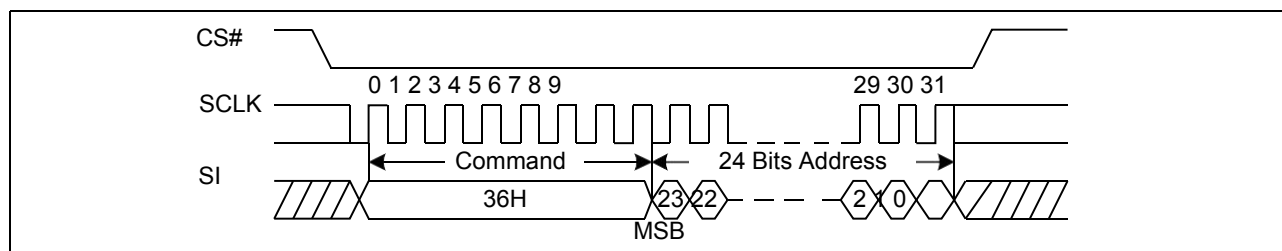
Figure34. Individual Block/Sector Lock command Sequence Diagram
