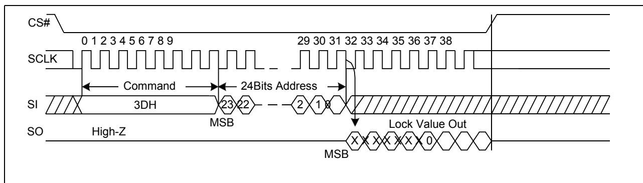
Figure36. Read Individual Block/Sector lock command Sequence Diagram
