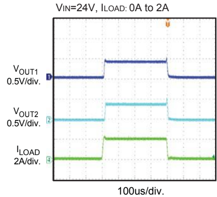
Transient Response
