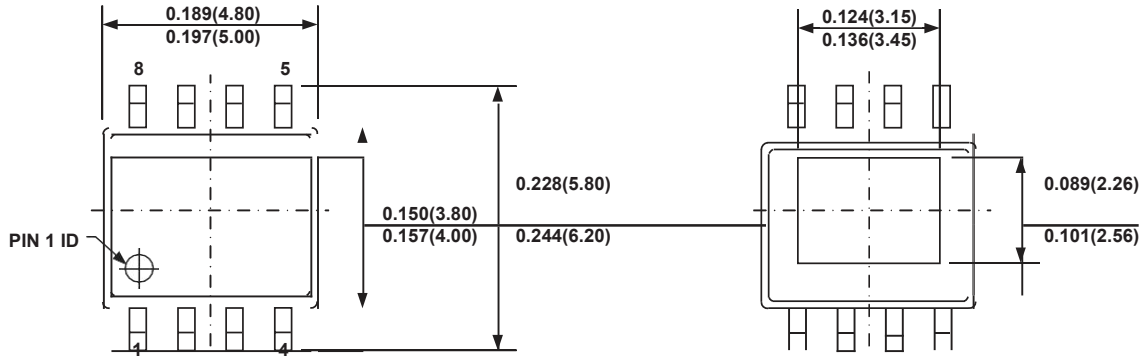
TOP VIEW
