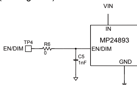
Figure 2: Analog Dimming External Circuit
