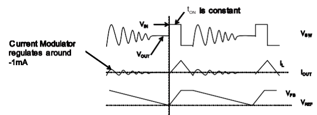
Figure 3: Light-Load Operation
