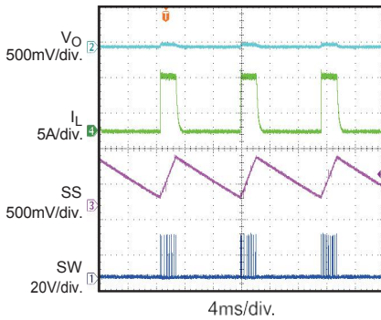
Short Circuit Recovery I_O = 5A
