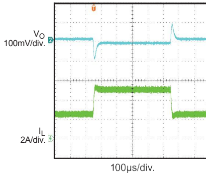
Load Transient I_O = 2.5A-5A@1.6\mu s
