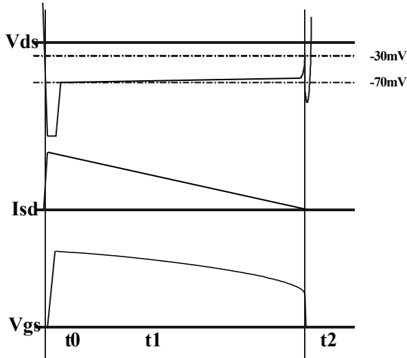
Figure 4—Synchronous Rectification Operation at light load SR Mosfet Selection and Driver ability
