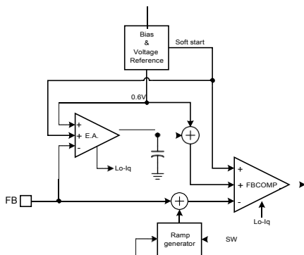
Figure 2: Operation Blocks at Sleep Mode
