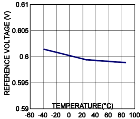
Reference Voltage vs. Temperature V_{IN} = 3.6V
