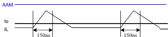
Figure 8: AAM Blank Time in Sleep Mode
